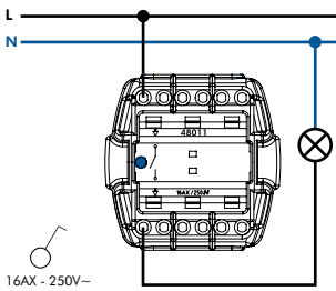
INTERRUPTOR BIPOLAR
